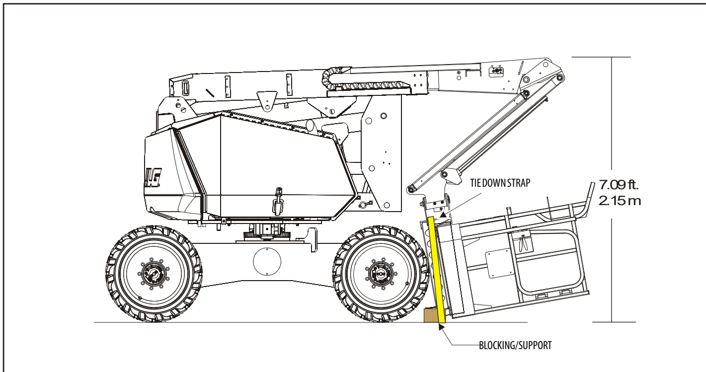
Figure 4-5. Storage Position
